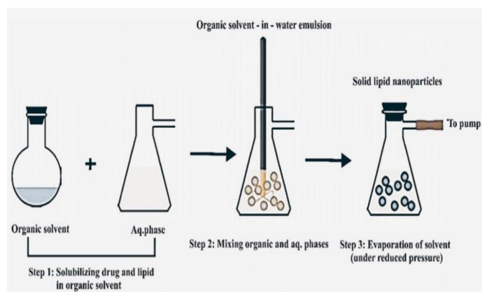
Fig.4 Solvent Emulsification/Evaporation
