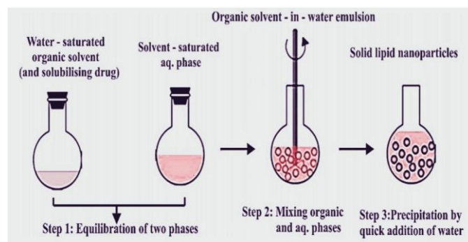
Fig.5 Solvent Emulsification/Diffusion
