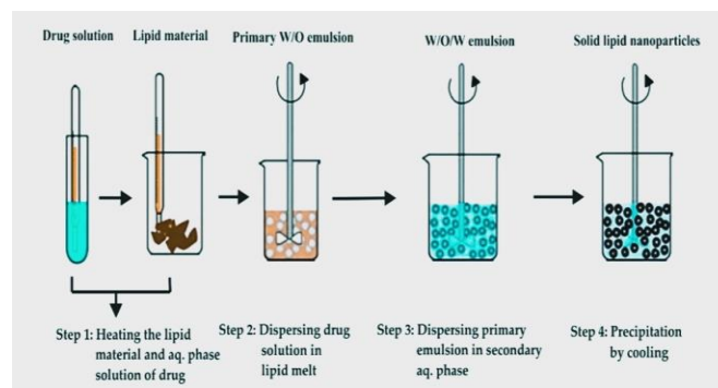
Fig.6 Double Emulsion
